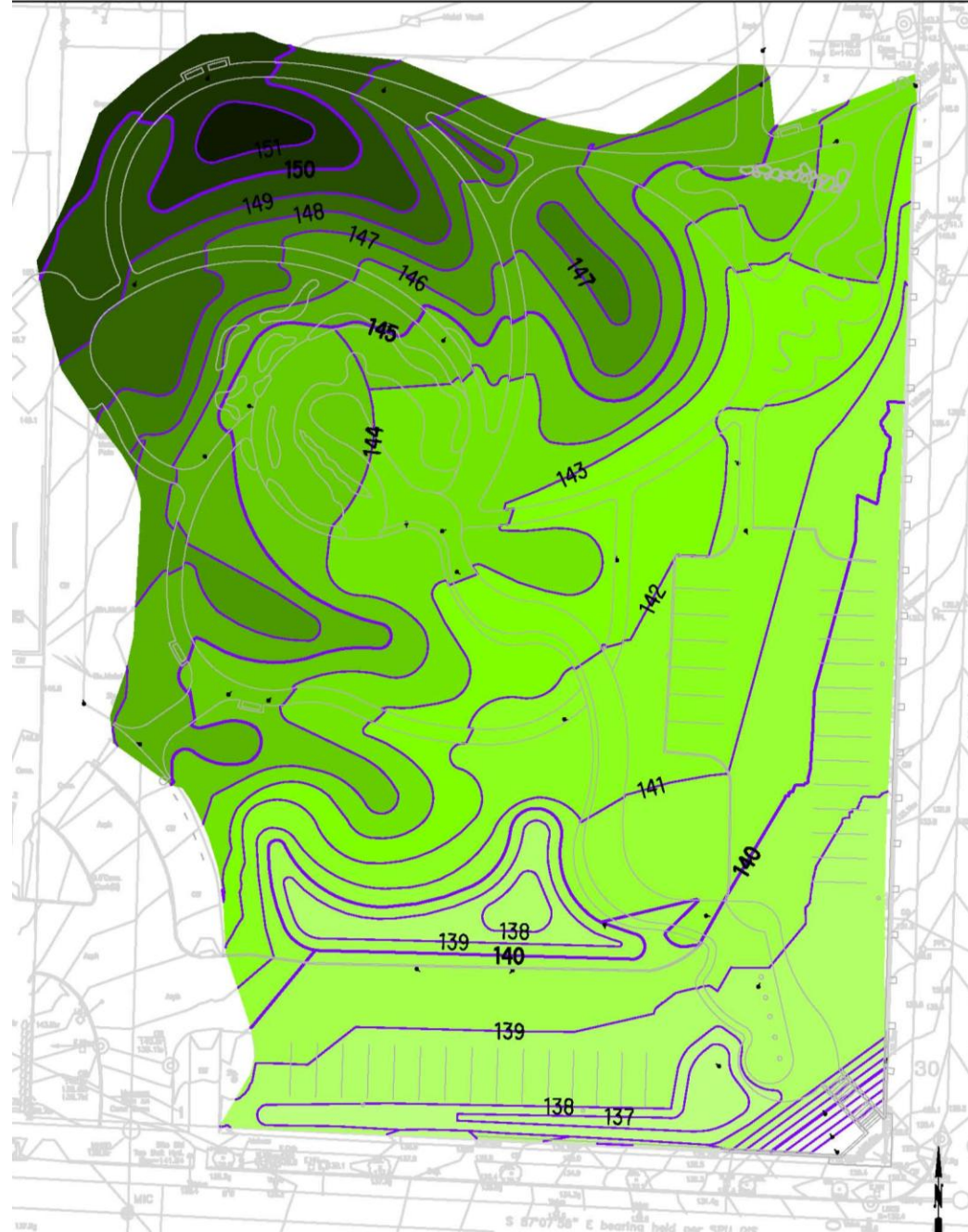
GRADING PLAN
